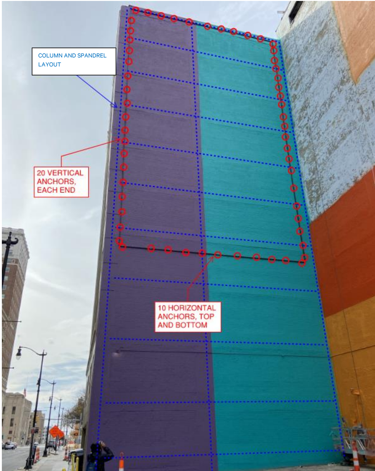
Figure 2 Wall Elevation (Photo by Silman)
