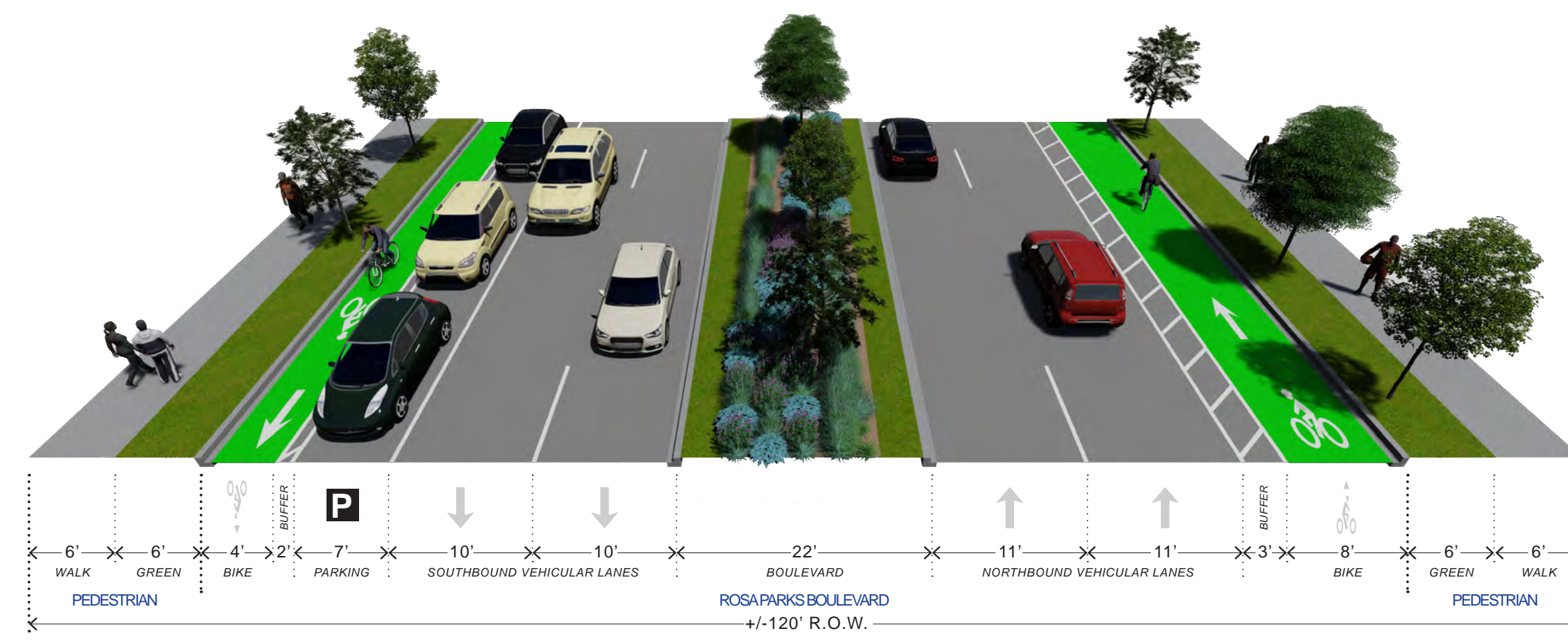
Proposed Improvements - On-street Parking
