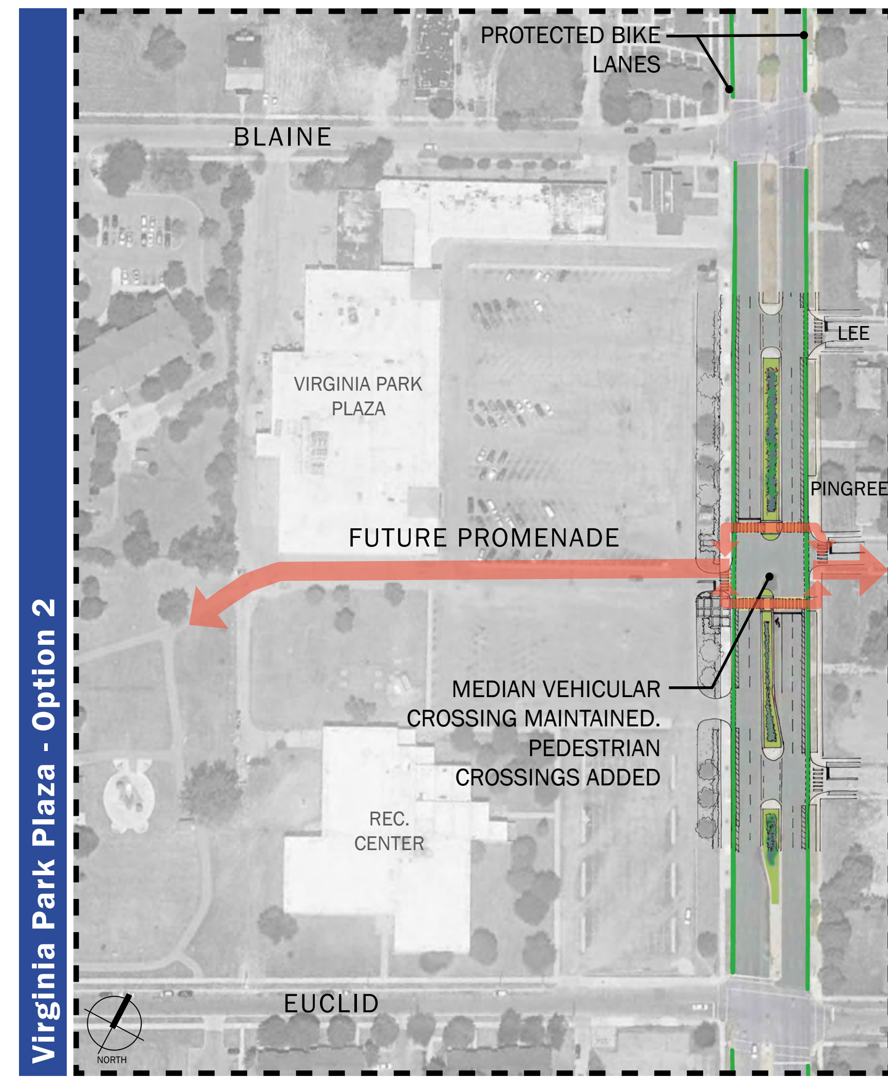
Proposed Improvements - No On-street Parking
